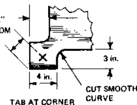
Fig. A. A dependable canopy to keep fallout and rain out of a vertical entry.
