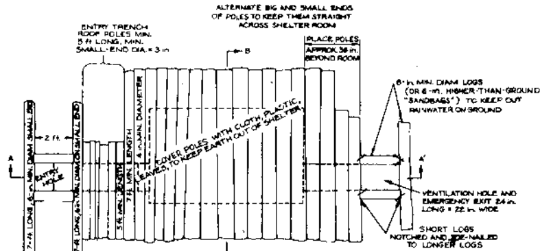
ROOF POLES - MINIMUM 7-ft LONG, 4-in. MINIMUM DIAMETER LAID ABOUT 2 ft. PAST EACH # 10 OF SHELTER ROOM. PLAN VIEW OF TOP OF SHELTER - SHOWING PLACEMENT OF POLES FOR ROOF (EARTH FILL NOT SHOWN)
