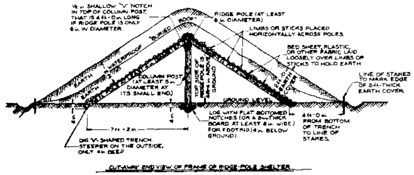
Fig. A.5. Aboveground, Ridgepole Shelter.
