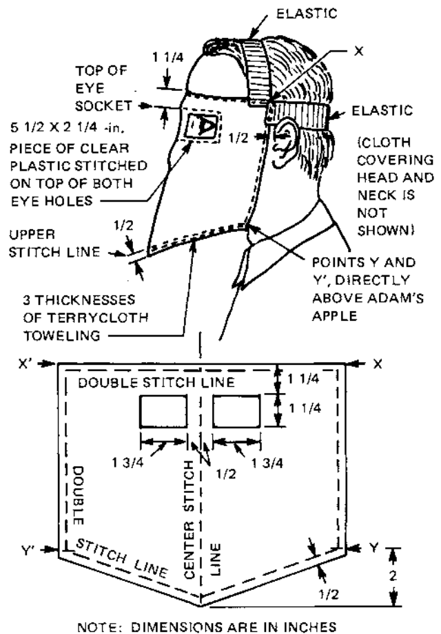
Fig. 15.9. A Russian-type homemade fallout mask. For most Americans this will continue to be a low-priority item as long as Russian warheads are large.
