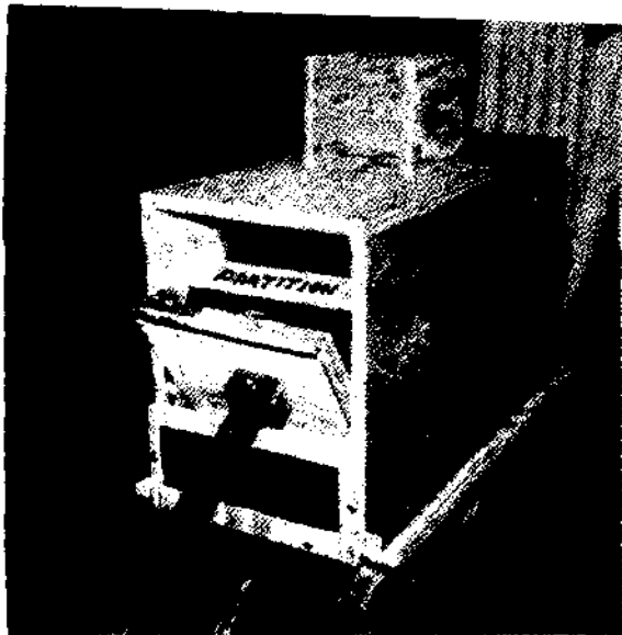
Fig. 6. Pump Built by Dale Huber, of Lake City, Florida in his home workshop, while guided only by the second draft of these repeatedly improved instructions. The removable part of the front end has been taken off, to insert the piston into the 12 x 12-in. "cylinder" under the PARTITION. The plastic flaps of this pump's flap valves are black transparent plastic film is preferred.
