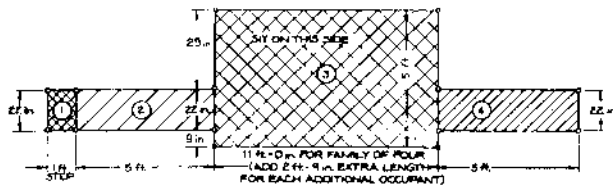
PLAN FOR STAKING OUT TRENCH ON TOP OF GROUND (SEE LEGEND FOR 4 DIFFERENT DEPTHS OF TRENCH) (FLOOR OF ROOM TRENCH = 3 ft - 6 in. WIDE)
