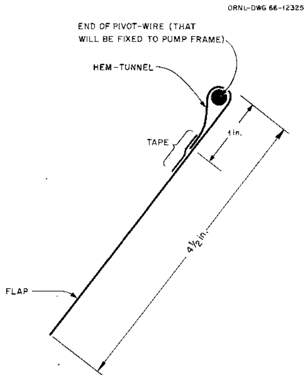
Fig. 7. End view.
