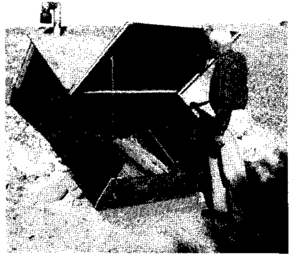
Fig. F.5. A Quickly Installable, 4-Piece Entryway Cover That Provides Easy Access and a Large, Protected Ventilation Opening.
