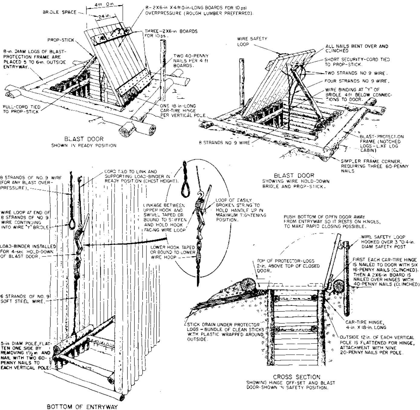
Fig. D.14. Expedient blast door that can be closed and secured in 4 seconds. Four seconds would be too little time if the shelter is at the 15-psi overpressure range from a 550-kiloton or smaller warhead — typical of the 1987 Soviet ICBM arsenal. (See the last paragraph on page 255.) However, this door closure is still the best blast-tested expedient means to secure a closed blast door.
