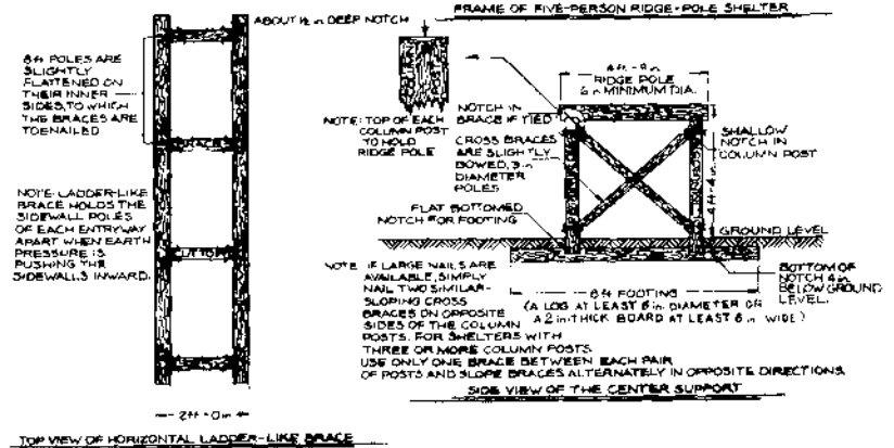
Fig. A.5. Aboveground, Ridgepole Shelter.
