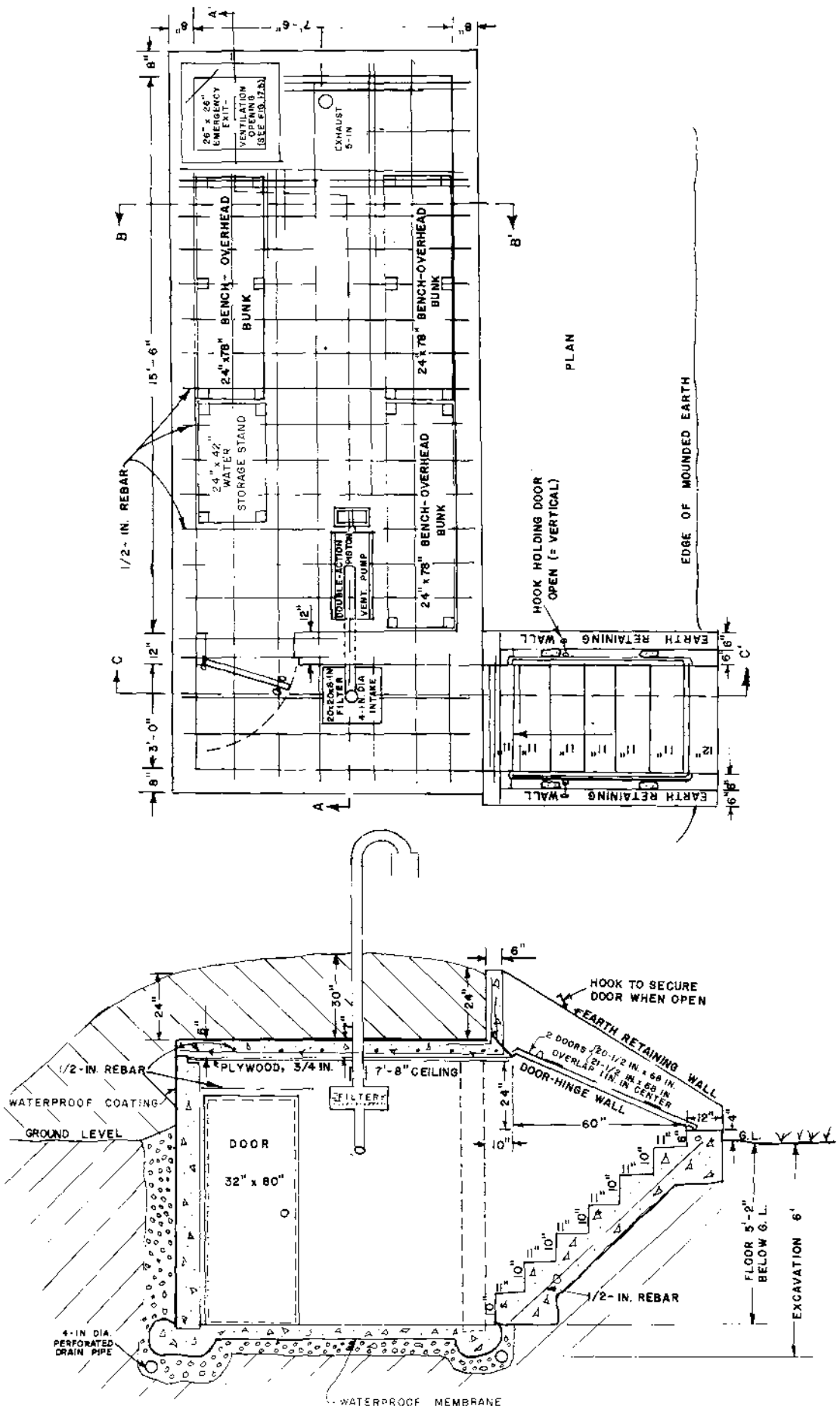
Fig. 17.1. Permanent Family Fallout Shelter for Dual Use.
