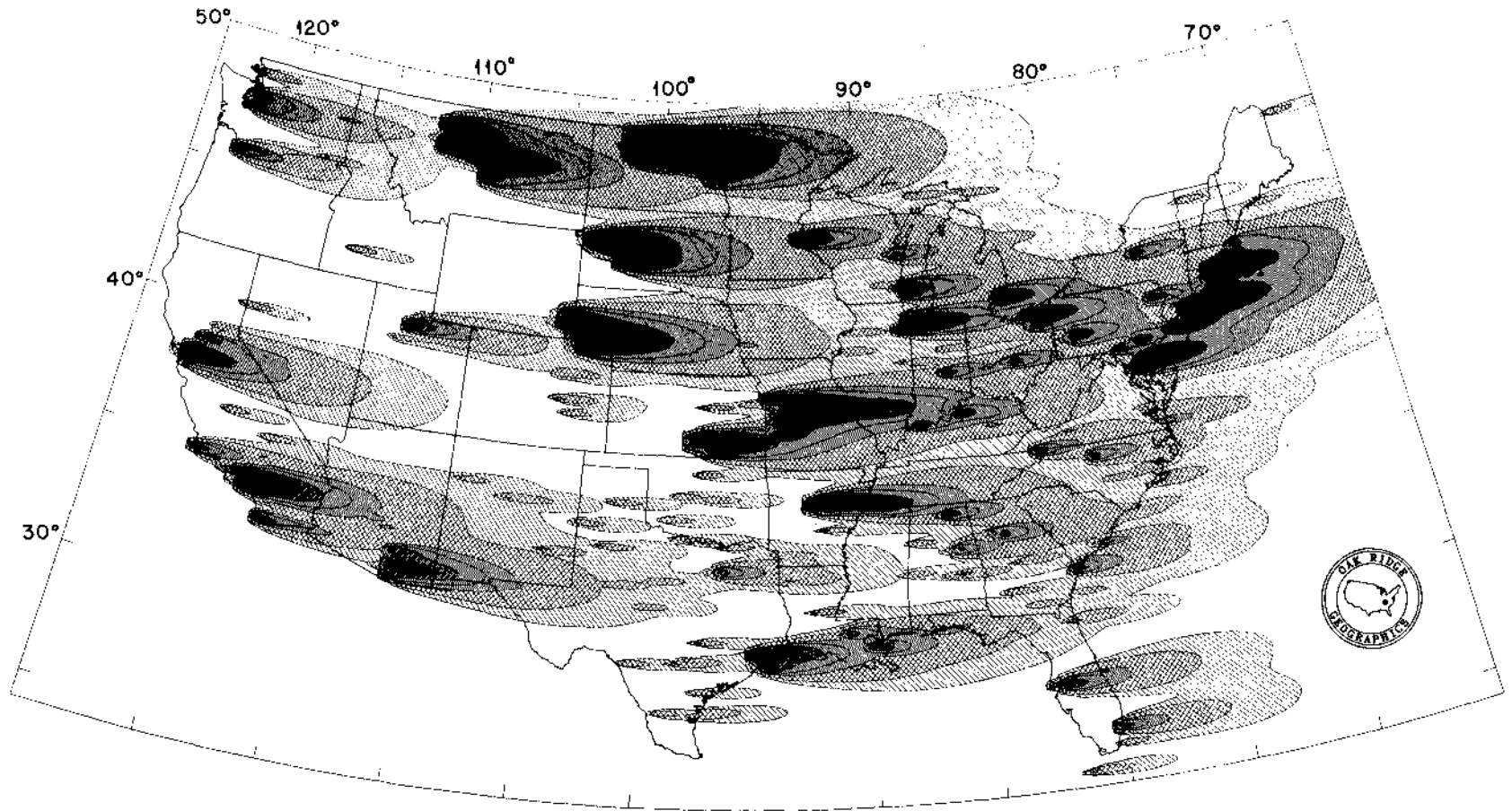
Fig. 4.2. Simplified, outdated fallout patterns showing total radiation doses that would be received by persons on the surface and in the open for the entire 14 days following the surface bursting of 5050 megatons on the targets indicated, if the winds at all elevations blew continuously from the west at 25 mph.
