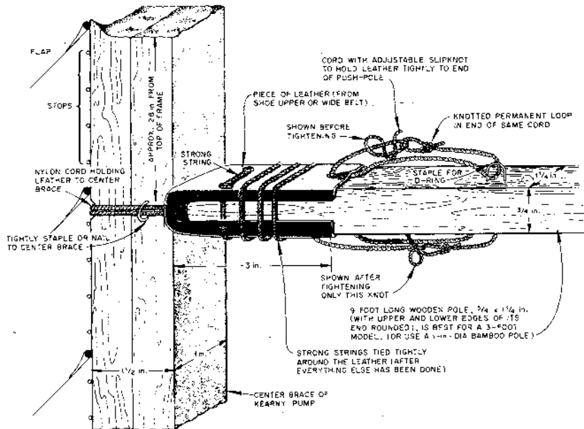
Fig. 26. Push-pole flexible connection.
